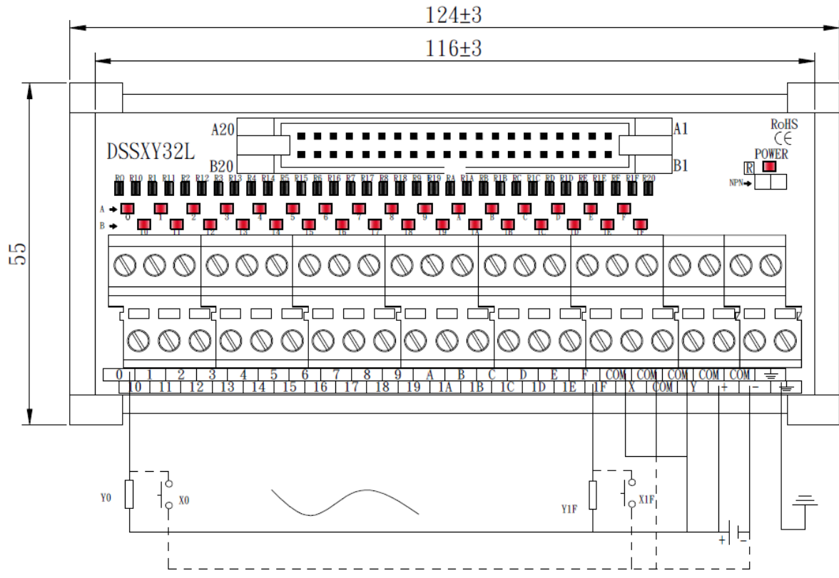
THIS DRAWING IS NPN OUTSIDE WIRING DIAGRAM
